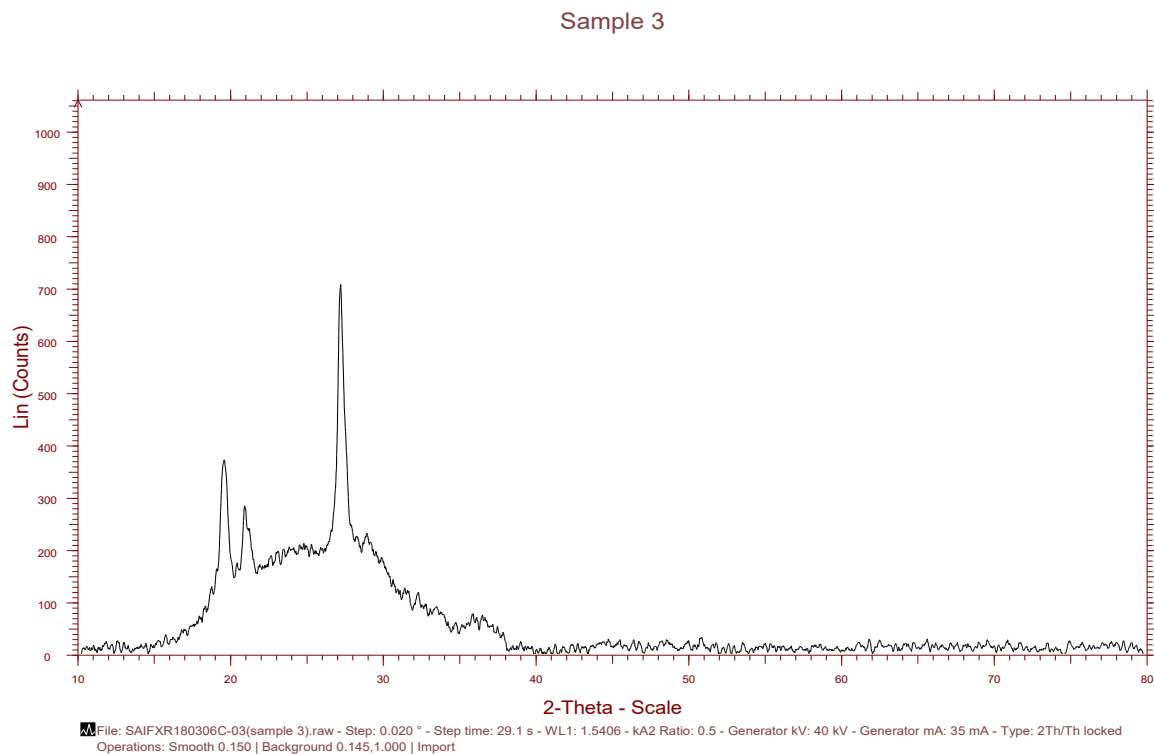
Figure.39 Zinc nanoparticle formation of (Sundari) dry fruit methanol extract under XRD imaging system.
